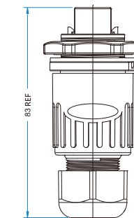
Dimensions figure
