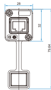
SX socket ( dimensions figure )
