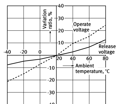
1-6. Ambient temperature characteristics (300 A Type)
