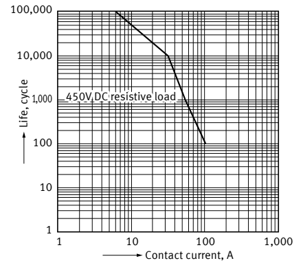
3. Switching life curve (Forward direction)
