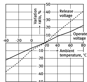
1-6. Ambient temperature characteristics (300 A Type)
