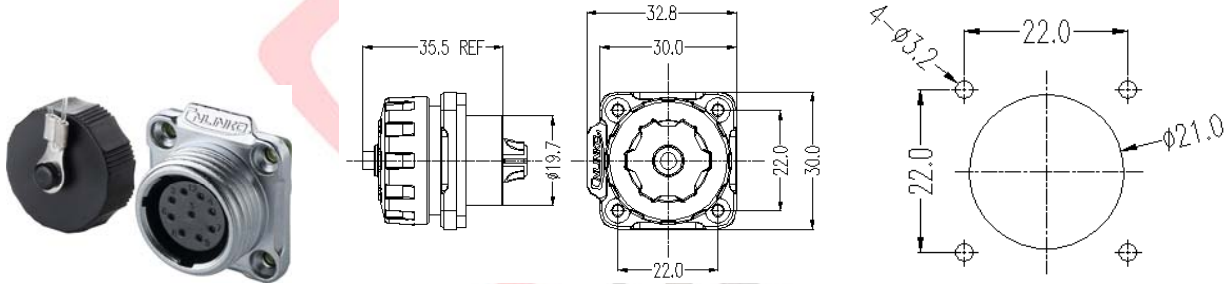
Mounting hole
