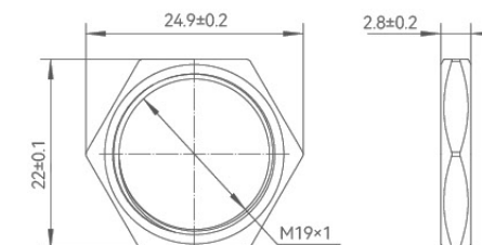
Attachment: Hexagonal Nut 附件: 六角螺母
