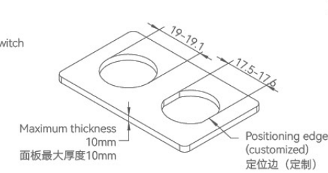
Panel opening size 面板开孔尺寸
