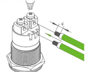
Diagram of wiring harness installation 线束安装图示 The maximum diameter of the threading hole is 2.4mm 穿线孔最大通过直径2.4mm
