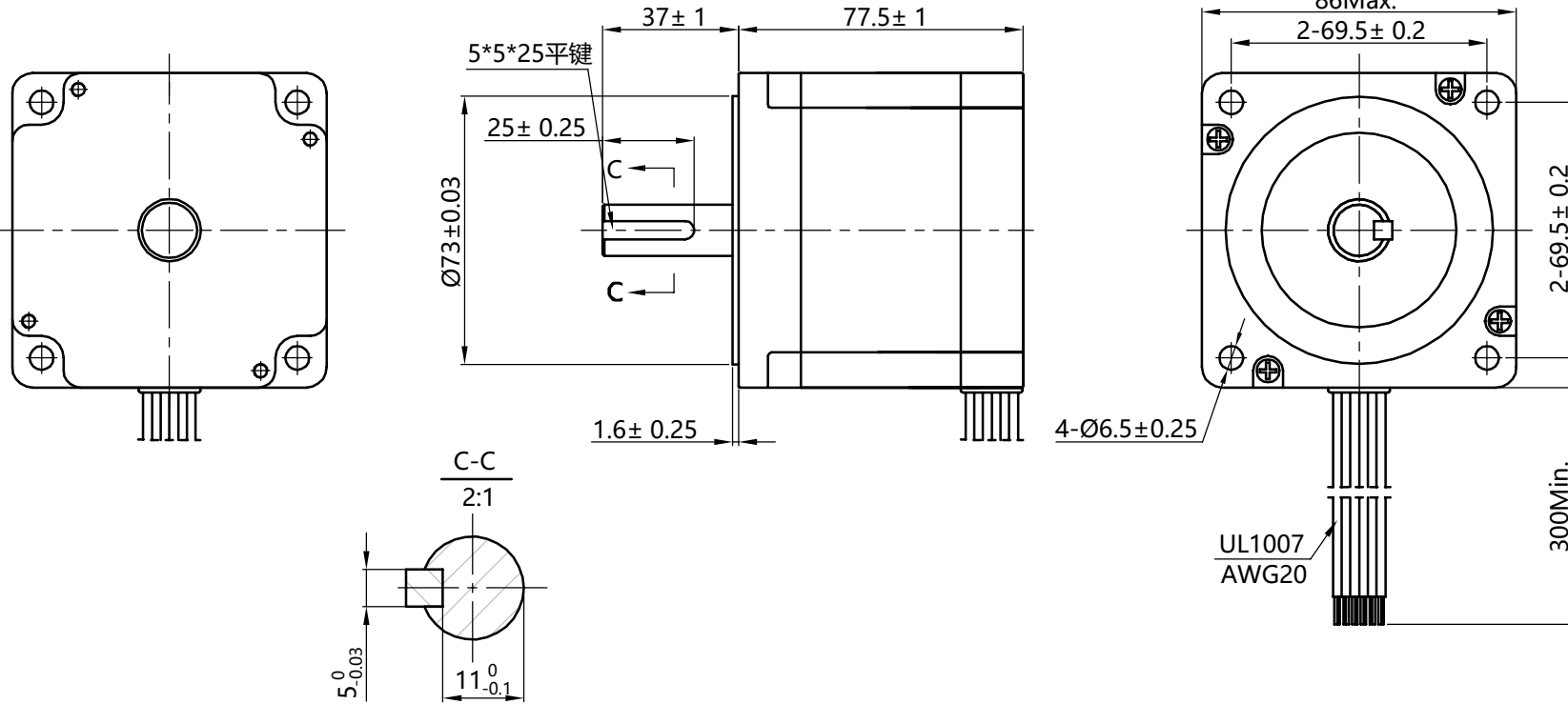
外形图 (DIMENSIONS) unit=mm
