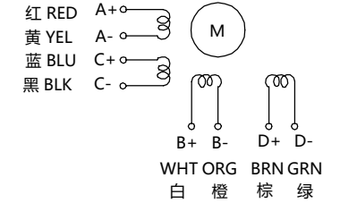
Wiring Diagram
