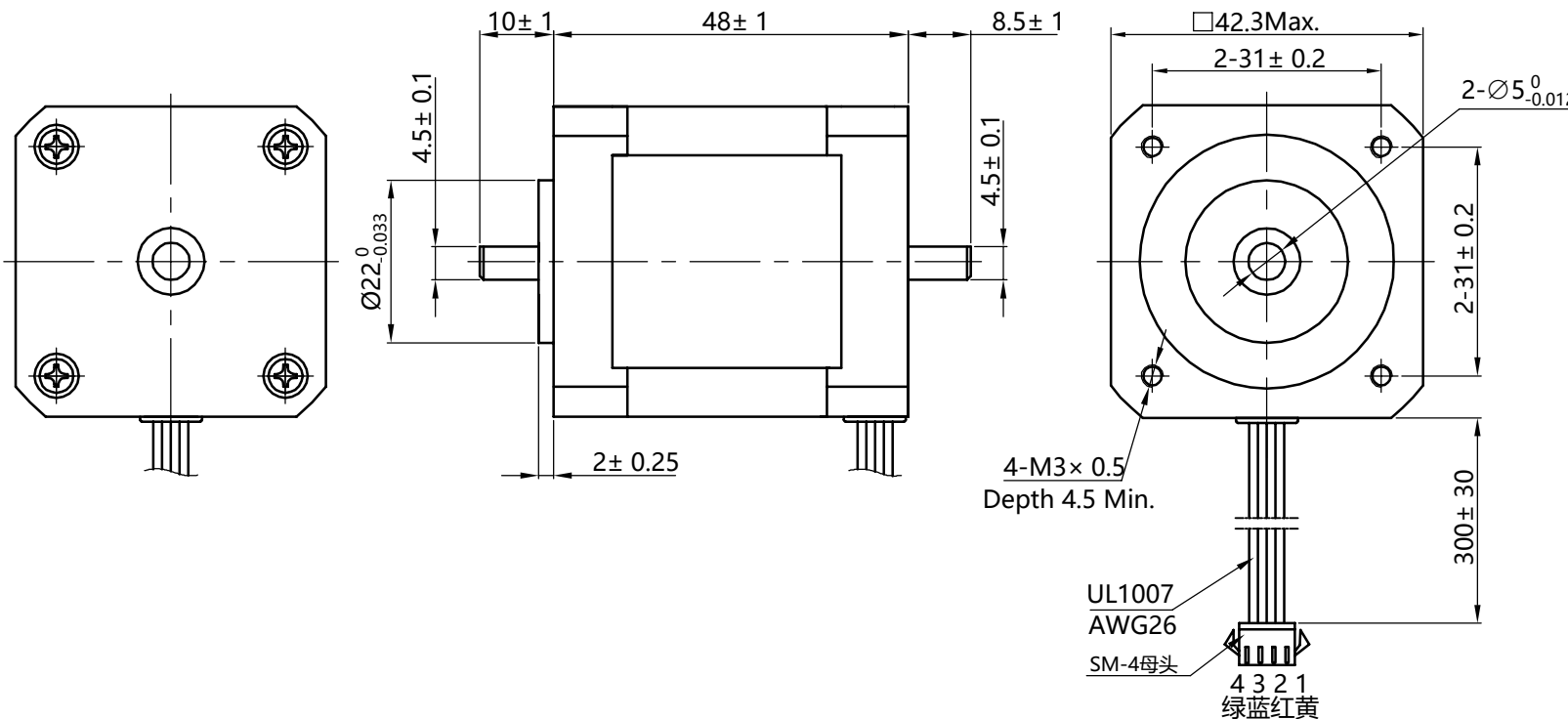
外形图 (DIMENSIONS) unit=mm
