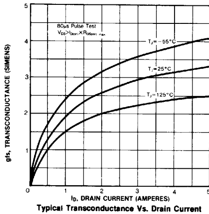
Typical Transconductance Vs. Drain Current
