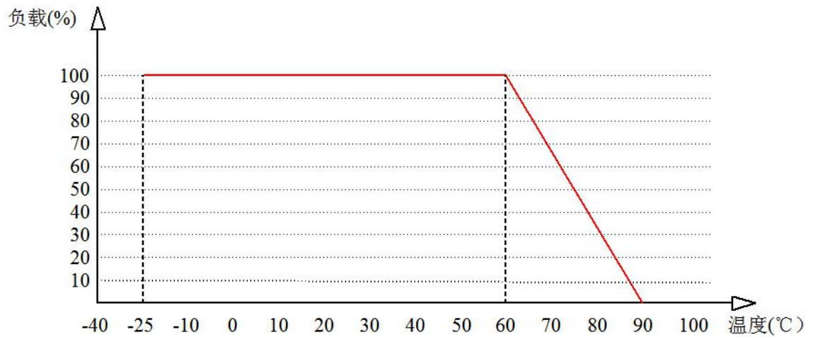
Working environment temperature and load characteristic curve
